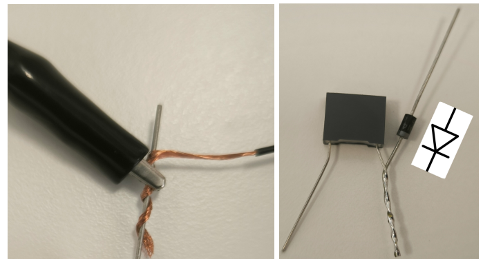
(a) Recommended electrical connection with wires wrapped to the capacitor with around another and secured with a crocodile clamp. (b) The diode attached with wires wrapped to the capacitor with around another and secured with a crocodile clamp, with the circuit symbol placed next to the diode in correct orientation.
